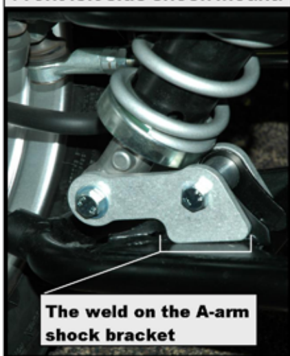
Front left side shock mount.
