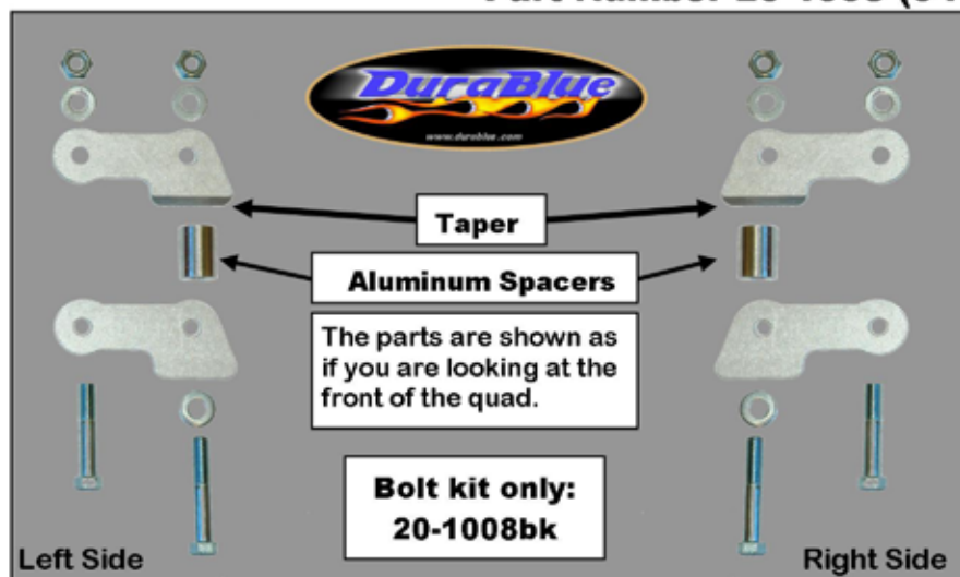
Front left side shock mount.
